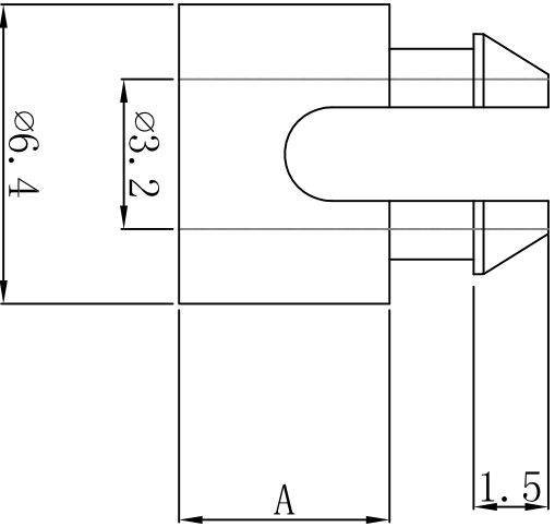
FOR #4 (M3) SCREW
